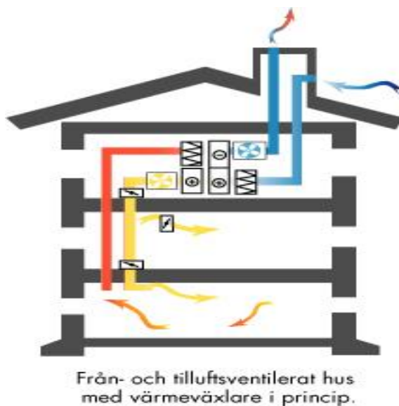
Figur 8: FTX-system 25
